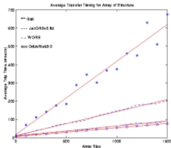
Figure 10: IOP communication performance for transferring a variable size array of structures by four Java ORBs: JacORB, JWORB, OrbixWeb and RMI. Poor RMI performance is due to the object serialization overhead, absent in the IOP/CDR protocol.
