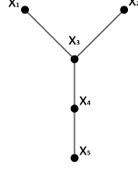
Figure 4.3: A tree G on 5 vertices
