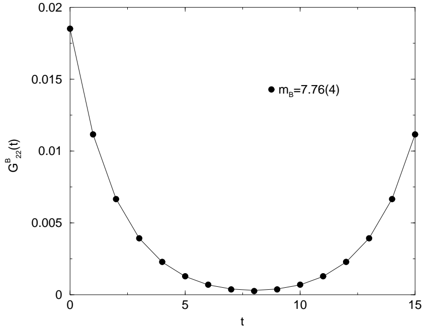
Figure 1: Boson Correlator at L = 16 and m = 10.0 , g = 3.0
