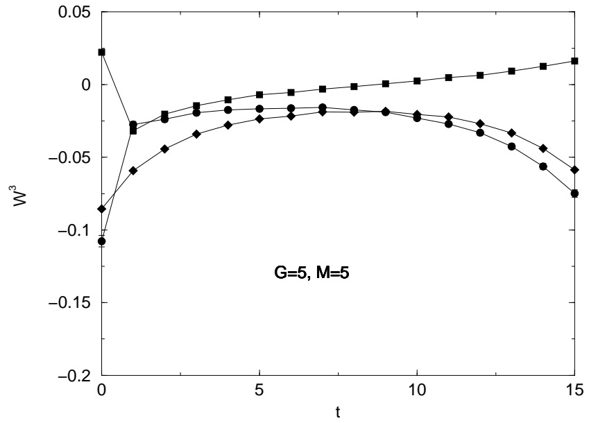
Figure 10: Fermionic and Bosonic Contributions to 3rd Ward identity for m = 5.0, g = 5.0, L = 16
