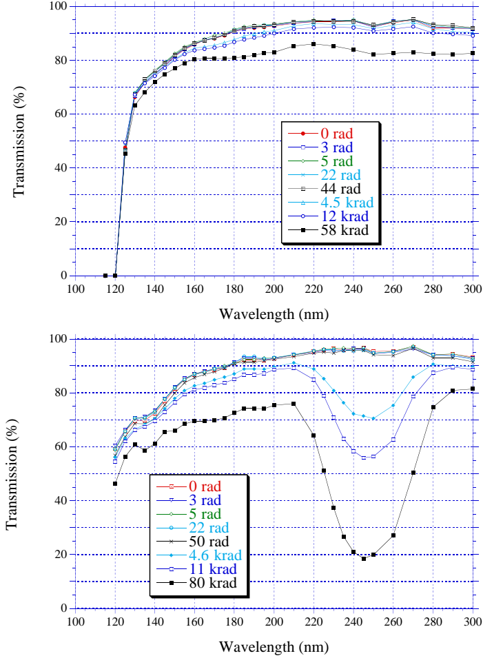
Fig. 14. Transmissions of CaF 2 (top) and LiF (bottom) crystal samples irradiated by a 60 Co source, for different exposures, up to 80 krad.
