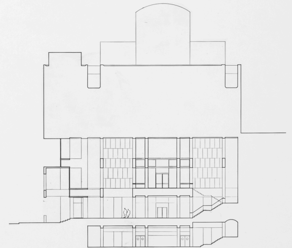
SECTION THROUGH ENTRY
