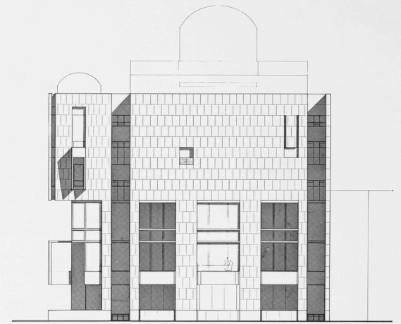
STREET ELEVATION
