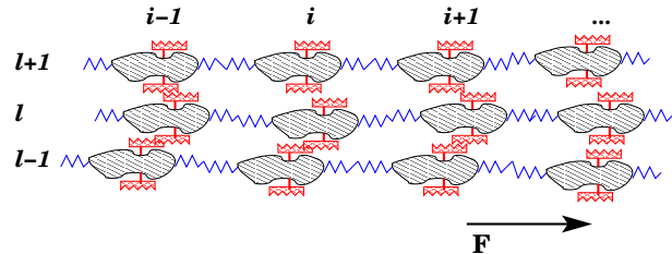
FIG. 1: A two-dimensional realization of the anisotropic driven medium described in the text. Degrees of freedom are labeled by discrete indices \ell and i , respectively transverse and longitudinal to the direction of the driving force, F . Each degree of freedom interacts with its neighbors via elastic couplings in the longitudinal direction and via viscous or similar slip couplings in the transverse direction.
