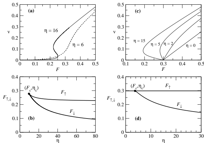
FIG. 2: Velocity curves and phase diagrams for the mean-field slip model. Part (a) shows the velocity v vs. force F curves for the purely viscous case for a broad distribution of pinning, \rho(h) = e^{-h} , for two values of viscous coupling \eta . Part (b) shows the phase diagram from (a), with curves indicating jumps in the adiabatic response (i.e., dv/dF \rightarrow \infty ) when the force F is increased from F = 0 ( F^\uparrow(\eta) ) and decreased from a sliding state ( F^\downarrow(\eta) ). The critical point (\eta_c, F_c) \approx (9.61, 0.278) . Part (c) shows example v vs. F curves when there is elasticity, K = 1 , for piecewise linear pinning forces and \rho(h) = e^{-h} . The curves are again continuous for \eta < \eta_c , but have a depinning transition at F_T , with critical behavior identical to the \eta = 0 case. When \eta > \eta_c , the depinning is abrupt and the v - F curves are hysteretic. Part (d) summarizes the K = 1 , \rho(h) = e^{-h} results in a phase diagram, indicating depinning from an initial pinned state at F^\uparrow = F_T and repinning from a sliding state at a lower force F^\downarrow(\eta) . The point (\eta_c, F_T) \approx (3.74, 0.298) is a tricritical point.
