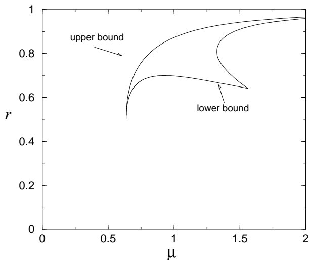
FIG. 7: Upper and lower bounds for r(u) , plotted as the coherence r(\mu = u/r) , corresponding to the maximal and minimal coherence static metastable states. The pinning force is taken to be piecewise linear with a = 1/\pi . A single static coherent solution is obtained only in the limit \mu \rightarrow \infty .
