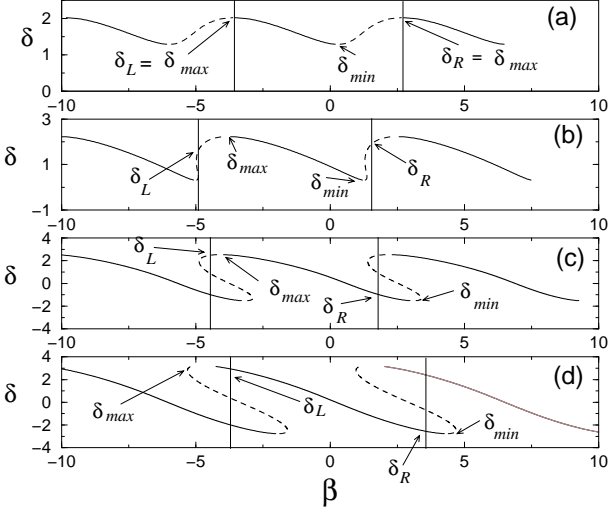
FIG. 26: The phase \delta as a function of \beta for various values of u and F < F_1^c(u) . Also shown in each frame are the values of \delta_{min} and \delta_{max} defined in Eq. (B4) and the boundary points \delta_R and \delta_L of the connected portion of the function \delta(\beta) that is used to evaluate the integrals determining the coherence in each case. The four curves corresponds to the four cases discussed in the text: (a) u < u_{sv}(F) , where \delta(\beta) is single-valued. In this case we can choose \delta_L = \delta_{max} , which requires \delta_R = \delta_{max} . As F is increased, \delta_{max} grows until \delta_{max} = \delta_L = \pi at F = F_1^c . (b) u_{sv}(F) < u \leq u_1(F) ; (c) u_1(F) < u \leq u_2(F) ; and (d) u > u_2(F) .
