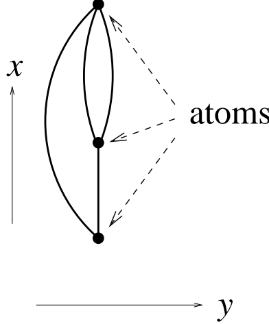
Fig.3: A molecule with 2 loops made of a connected assembly of 4 dipoles. This molecule has 3 atoms located at different values of x but at the same value of y .
