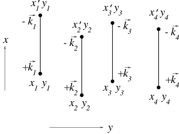
Fig.2: The diagram of order N in (3.2) is made of N dipoles. The two end points of a given dipole are located at the same position y_i in the y direction but at different positions x_i and x'_i in the x direction.
