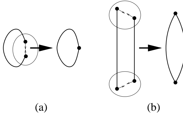
Fig.4: The two singular configurations leading to (a) a one loop renormalization of (\partial_x \vec{h})^2 and (b) a one loop renormalization of \delta^{(d-1)} \left( \vec{h}(x, y) - \vec{h}(x', y) \right) .
