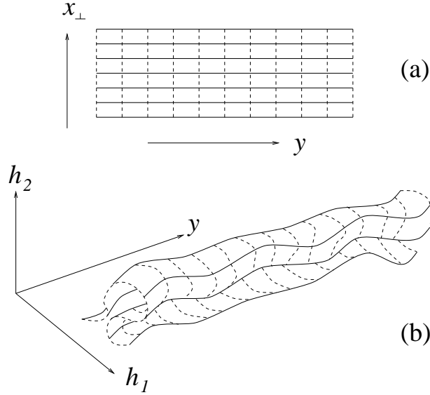
Fig.1: (a) An anisotropic membrane with a stiff y direction and a soft x_{\perp} direction; (b) after embedding, the membrane forms a tubule, extended in the stiff y direction and crumpled in the soft direction.
