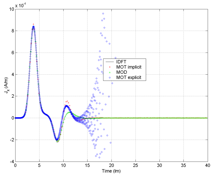
Figure 4. The induced current across edge 67 of the cone.
