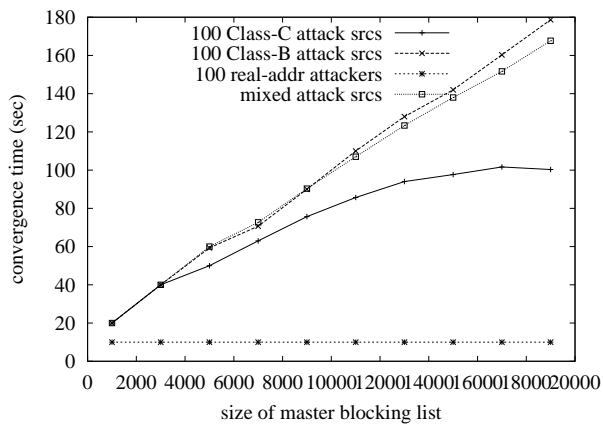
Fig. 4. Convergence time with respect to firewall configuration
