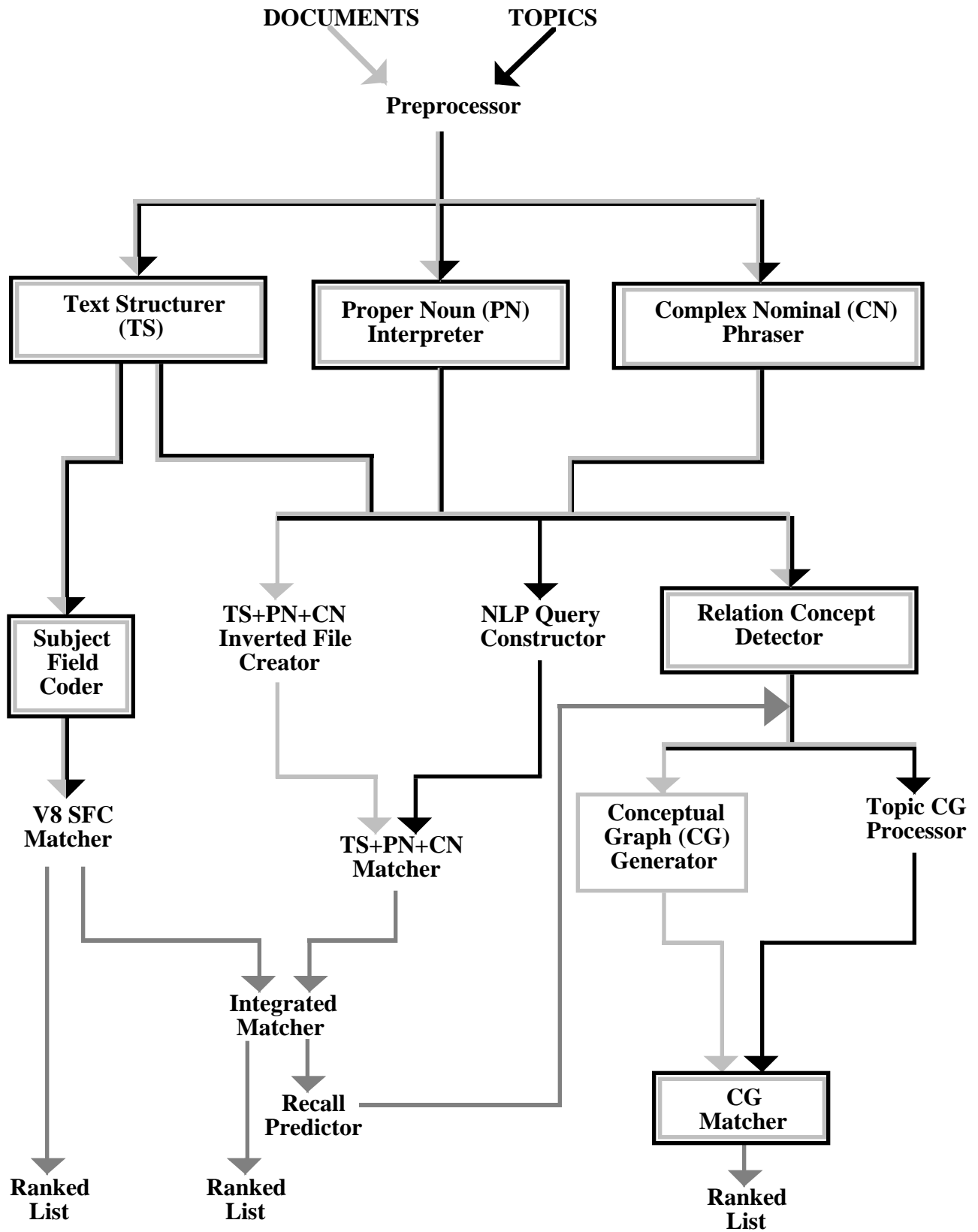
Fig. 1: DR-LINK System
