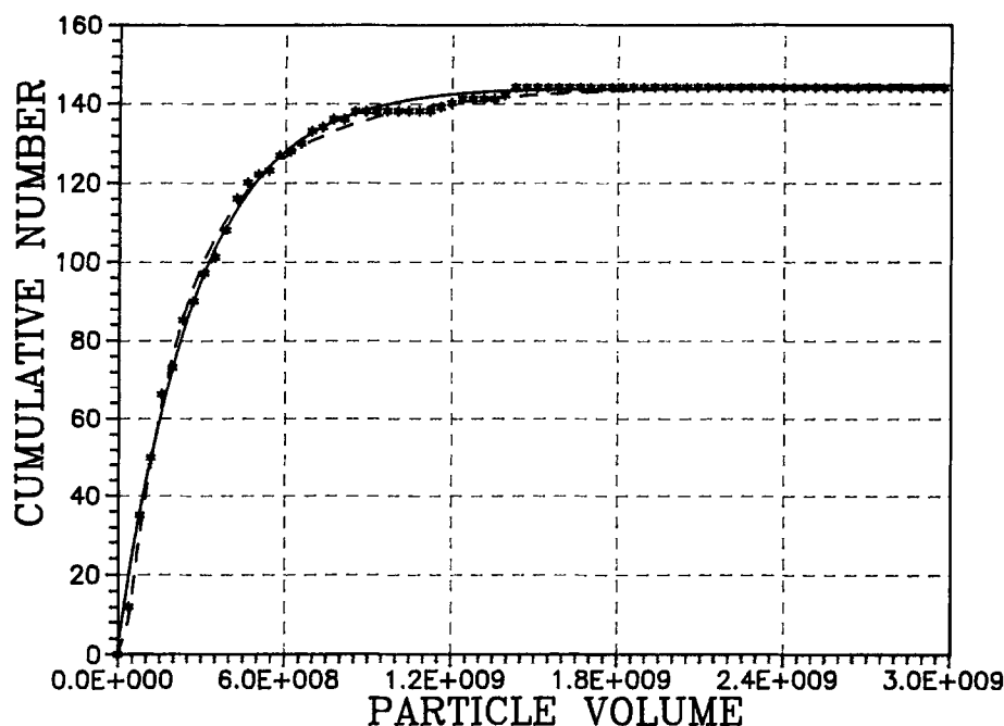
Fig. 1. Fit of film Al10 cumulative number data (*) to log-normal (---) and Poisson distributions (—).
