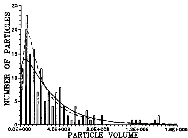
Fig. 2. Poisson and log-normal distributions for film Al10 data compared with histogram of volumes.
