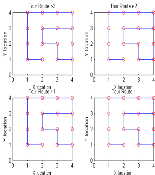
Figure 8. Optimal route in Wireless Sensor Network - with 16 Nodes using Ant System [Q: 0.9 Rho: 0.7 Alpha: 4 Beta:7]
