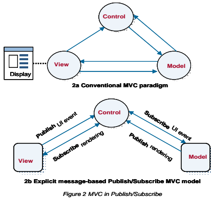
Figure 2. MVC in Publish/Subscribe
