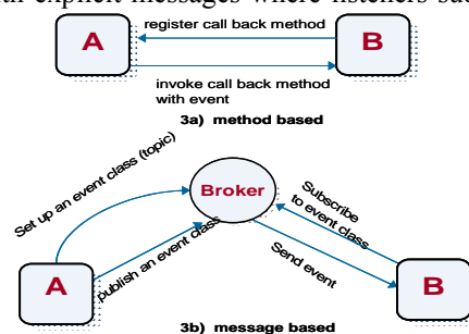
Figure 3 Message or method based Publish/Subscribe
