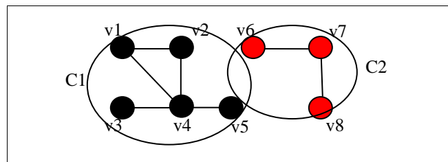
Figure 5. Example DSG
