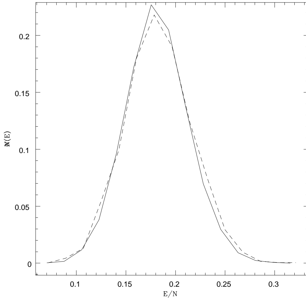
Figure 13: The number of solutions of the T = 0 mean field equations of a given energy as function of the energy for N = 56 , where (2N + 1) is prime (dashed line) and for N = 57 , where (2N + 1) is not prime (continuous line).
