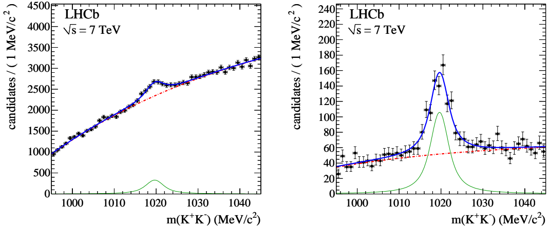
Figure 1: Fit to the tag (left) and the probe (right) sample in the bin 0.6 < p_T < 0.8 \text{ GeV}/c , 3.34 < y < 3.52 for one of the two magnet polarities. Shown are the data points, the fit result (thick solid line) as well as the signal (thin solid line) and the background component (dash-dotted line).
