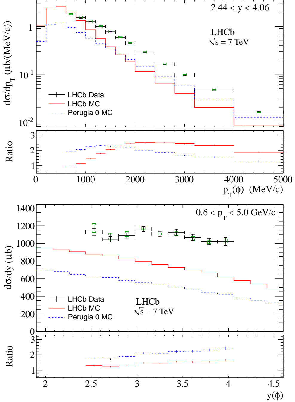
Figure 2: Inclusive differential \phi production cross-section as a function of p_T (top) and y (bottom), measured with data (points), and compared to the LHCb default MC tuning (solid line) and Perugia 0 tuning (dashed line). The error bars represent the statistical uncertainty, the braces show the bin dependent systematic errors, the overall scale uncertainty from Table 1 is not plotted. The lower parts of the plots show the ratio data cross-section over Monte Carlo cross-section. Error bars in the ratio plots show statistical uncertainties only.
