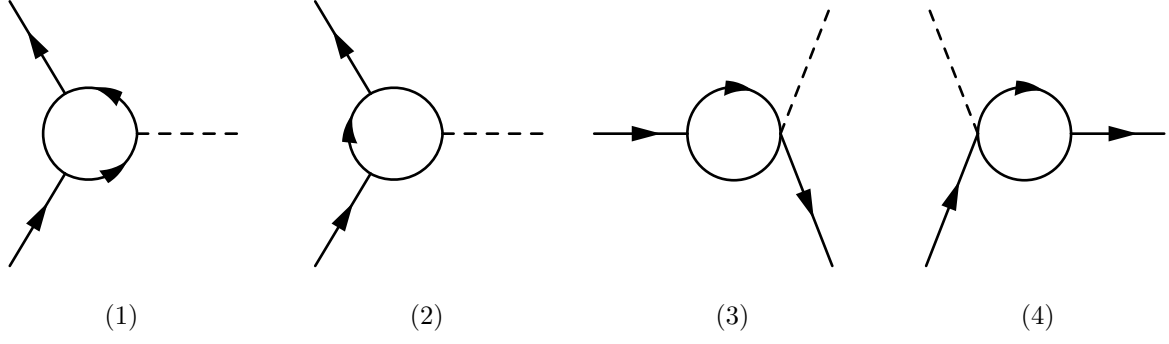
FIG. 4: One-loop corrections to the vertex for scalar emission by matter
