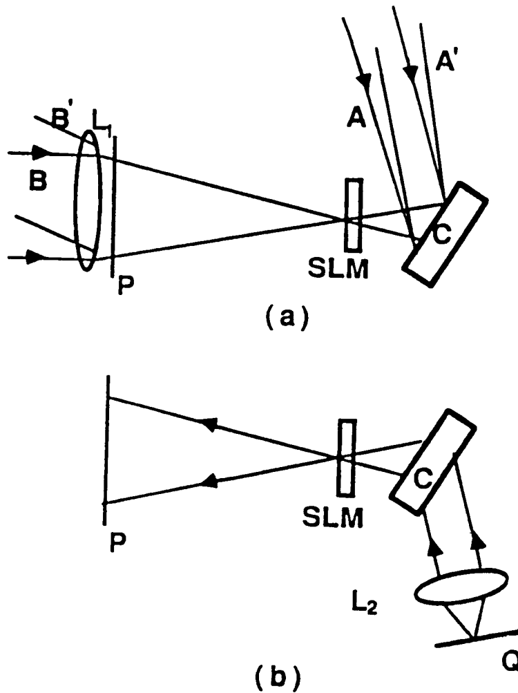
Figure 5: Geometry for Reconfigurable Interconnections with Spatial Division (a) recording setup (b) Reading Setup
